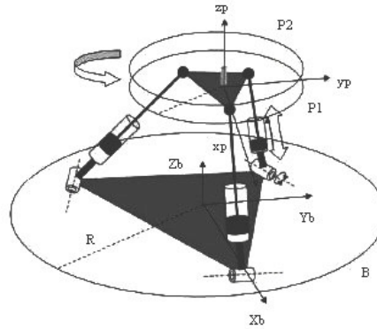
Figure 3. Tripod based ankle rehabilitation device.
