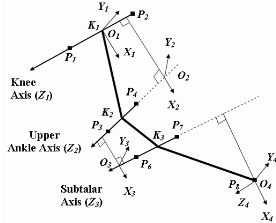
Figure 6. Serial kinematics chain of the foot and D-H frames assignment.
