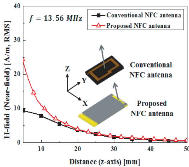
Figure 4. Simulated H -field (near-field) intensity with a normal direction ( z -axis) at the center of the proposed NFC antenna and the conventional 4-turn NFC loop antenna at 13.56 MHz.
