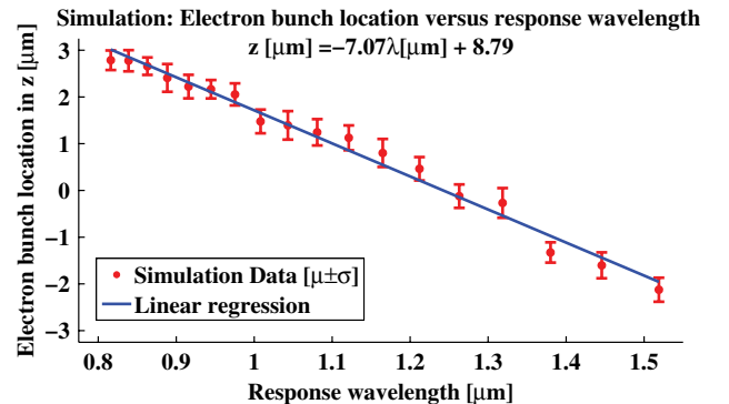
Fig. 4. (Color online) Simulation of the electron bunch z location versus the clamshell BPM response wavelength. The markers define the center of the excitation channel as determined by a Gaussian fit to the simulation data, whereas the error bars represent the width of the Gaussian fit.
