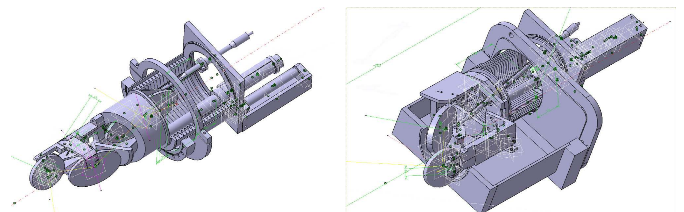
Sketch of the present design of the ports. In the picture are depicted the mirrors, the vacuum interface window, the translation stage on bellows and the screw actuator used to adjust the orientation of the plasma-facing mirror
