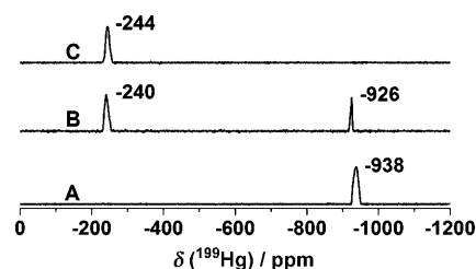
Figure 2. 199 Hg NMR spectra of solutions containing \alpha_3 DIV (2.93 mM) and 199 Hg(NO 3 ) 2 (0.8 equiv) at pH 5.8 (A), 7.4 (B), and 8.6 (C).
