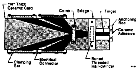
Fig. 4. Wire target array on its ceramic card.
