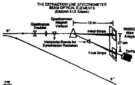
Fig. 1. Schematic diagram of the (electron) extraction-line spectrometer beam optics and synchrotron beams.
