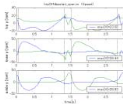
(b) Angular Velocity of Pitch Axis
