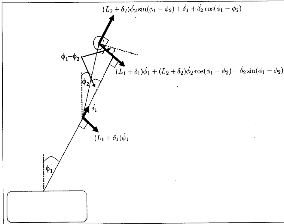
Figure 4.3: System Velocities
