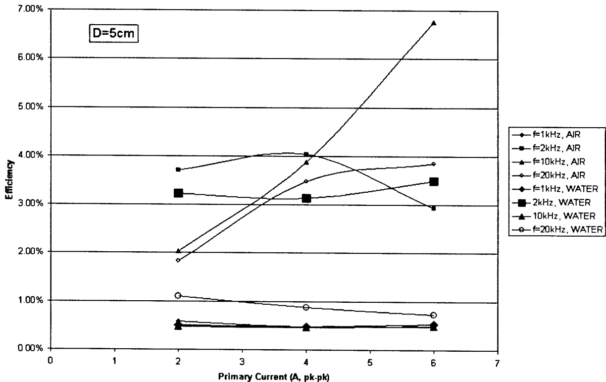
Figure 6.6: Efficiency vs. Primary Current
