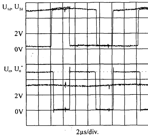
Fig. 8. Principle operation of PLL ( \phi \approx 0^\circ , \theta \approx 68^\circ )
