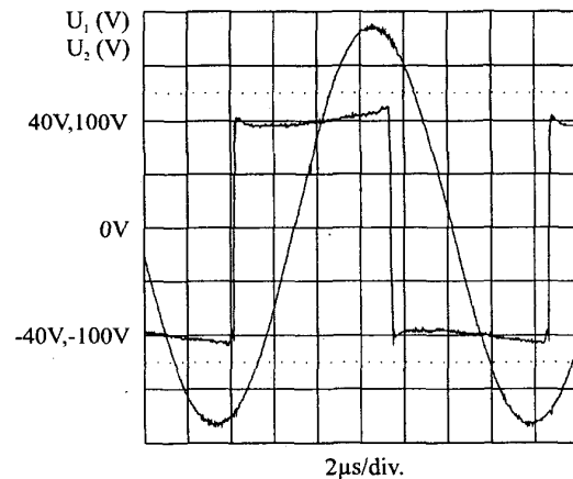
Fig. 9. Current I_1 and voltages U_1 , U_2 for \phi \approx 0^\circ , \theta \approx 68^\circ
