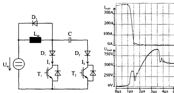
Fig. 2. IGBT turn off measured on a current source ZVS test bench
