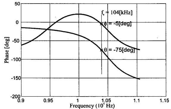
Fig. 6. Relation between the phase \phi(I_1/U_1) and the phase \theta(U_2/U_1) of the LCLR-tank
