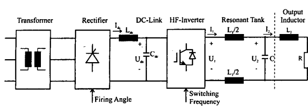
Fig. 3. High-frequency induction heating system with LCL-resonant output
