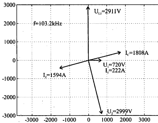
Fig. 5. Phasor diagram for rated power, load 2
