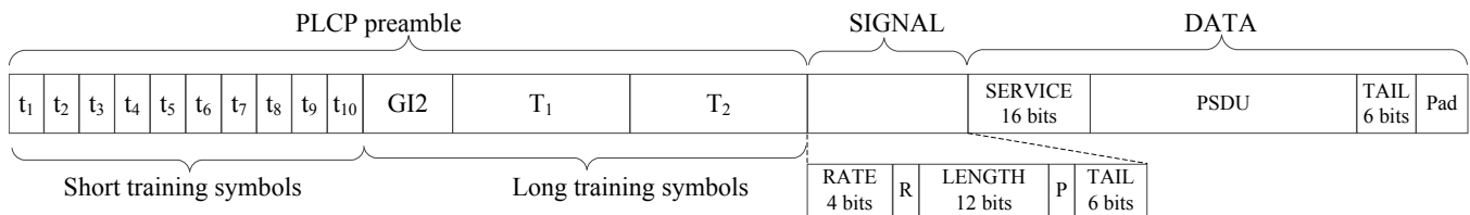
Fig. 7. IEEE 802.11 OFDM PPDU frame format [24] (For simplicity, guard interval of the OFDM data symbols is not shown in the figure)
