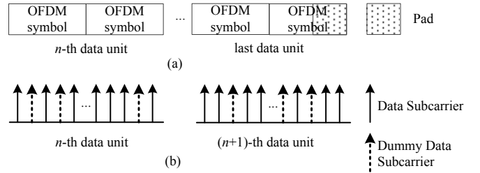
Fig. 3. Illustration of the data unit. (a) Example of the data unit structure ( s = 2 ); (b) Example of the dummy data subcarrier obfuscation ( s = 2 , k = 3 )
