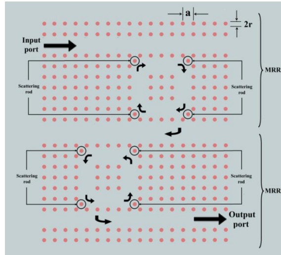
Fig.6. Proposed structure of serially cascaded PhC based double MRR
