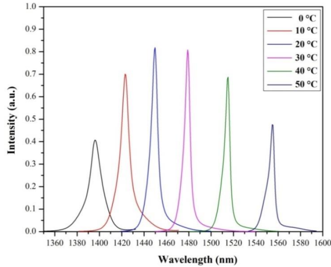
Fig.5. Output normalized intensity at different temperatures of single MRR structure at the drop port
