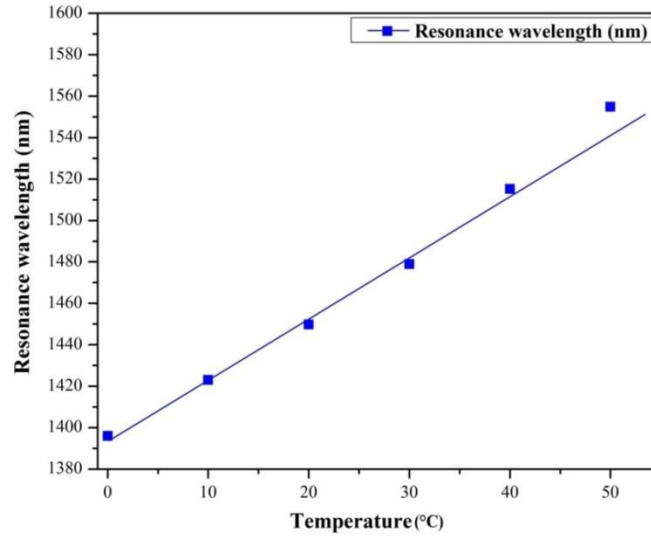
Fig.8. Sensitivity graph of single MRR structure
