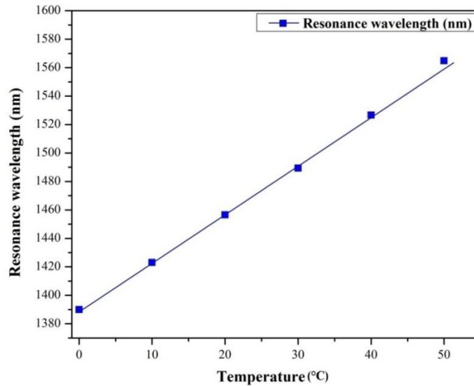
Fig.9. Sensitivity graph of cascaded MRR structure
