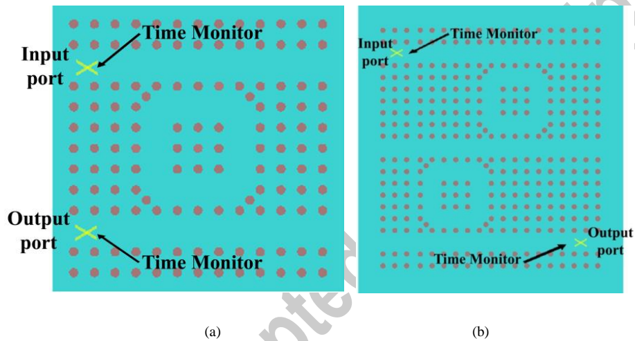
Fig.10. Schematic diagram of (a). Single MRR structure (b). Cascaded MRR structure to calculate the response time
