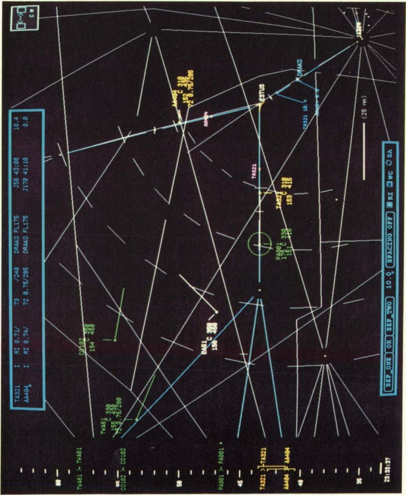
Figure 4.- Integrated controller display with spacing advisories.
