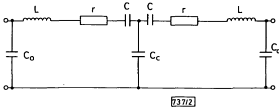
Fig. 2 Electrical equivalent circuit of one m.c.f.
