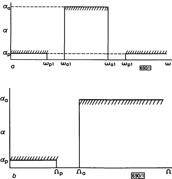
Fig. 1 a Bandstop filter specifications b Lowpass prototype specifications
