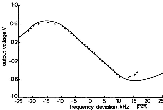
Fig. 3 Discriminator output characteristic — theoretical; + experimental. Centre frequency 10.7 MHz, input signal 1 V r.m.s.
