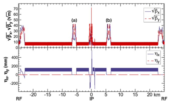
FIG. 5. The beam optics of the FCC-ee half ring, corresponding to \beta_{x,y}^* = (1 \text{ m}, 2 \text{ mm}) . Upper/lower plots show \sqrt{\beta_{x,y}} and horizontal/vertical dispersions, respectively. These plots start and end in the middle of the rf sections, and the IP is located at the center. Sections marked by (a,b) correspond to the intermediate straight sections B, F, H, L in Fig. 1.
