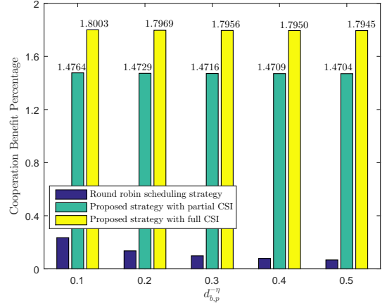
Fig. 8. Cooperation benefit percentage \Lambda as a function of d_{b,p}^{-\eta} achieved by different secondary user scheduling strategies, \rho = 25 dB, N = 3 .
