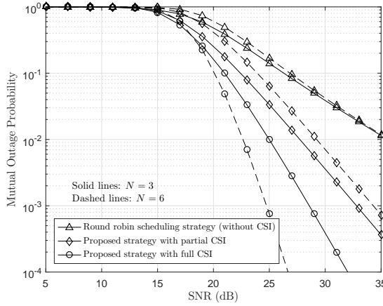
Fig. 7. Mutual outage probability achieved by different secondary user scheduling strategies, R_p = 1 bits/Hz, R_s = 1.5 bits/Hz.
