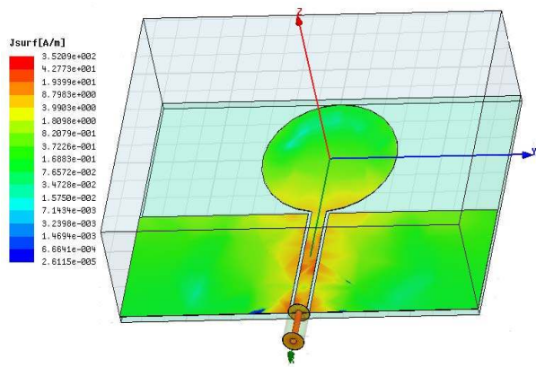
Fig. 3. Current Distribution on the monopole Patch Antenna
