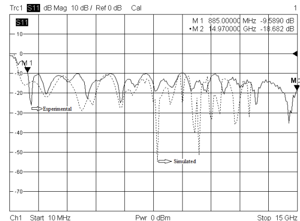
Fig. 9. Experimental and simulated results of fractal antenna
