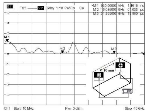
Fig. 17. Group Delay of fourth iterative circular shape fractal antenna
