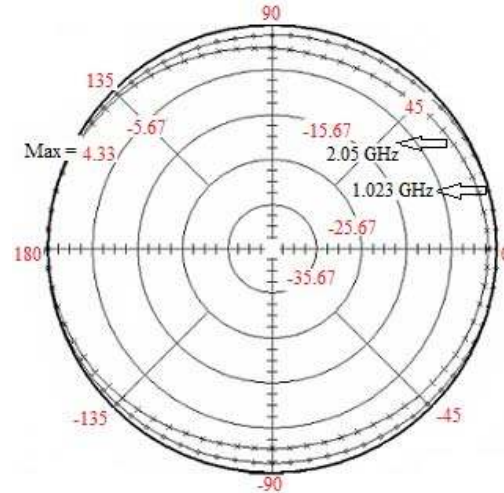
Fig. 12. Experimental radiation pattern of fractal antenna at frequency at 1.023-1.683 GHz
