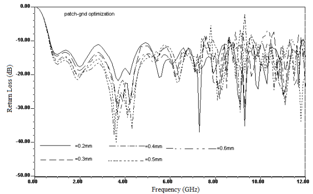
Fig. 5. Simulated result of fractal antenna with respect to gap between ground plane and patch
