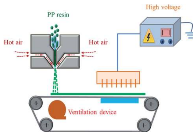
Fig. 1 Schematic illustration of the fabrication procedure of the PP melt blown nonwovens and the corona charging technology.
