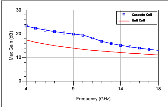
Fig. 6 Comparison of maximum available gain on 4-18GHz between the balanced cascode cell and a single transistor with input (Cag // Rag) cell.
