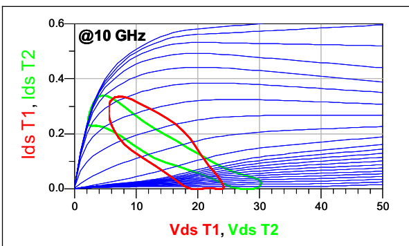
Fig. 8 Intrinsic load lines of each transistor of the cascode cell @ 10.24GHz
