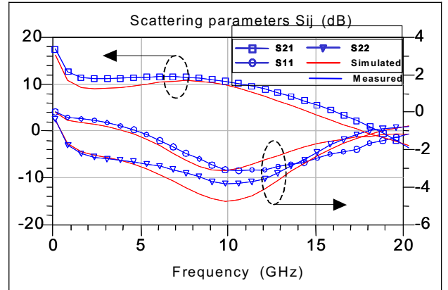
Fig. 9 Comparison between simulated and measured scattering parameters of the balanced cascode cell at V_{BIAS\_D}=30 V, V_{BIAS\_G1}=-6 V, and V_{BIAS\_G2}=9 V
