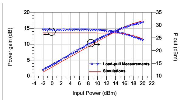
Fig. 11 Comparison between simulated and measured large signal results for the cascode cell with (20+j.12) load impedance @ 10.24 GHz
