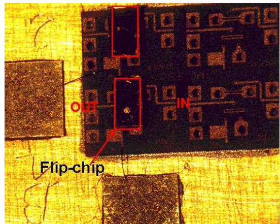
Fig. 5 Photograph of two GaN cascode flip-chipped onto AlN substrate for on-wafer measurements.
