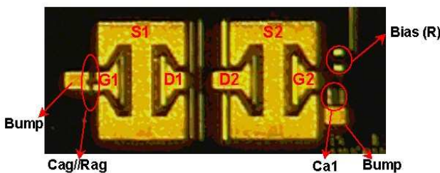
Fig. 3 Photograph of the GaN cascode cell
