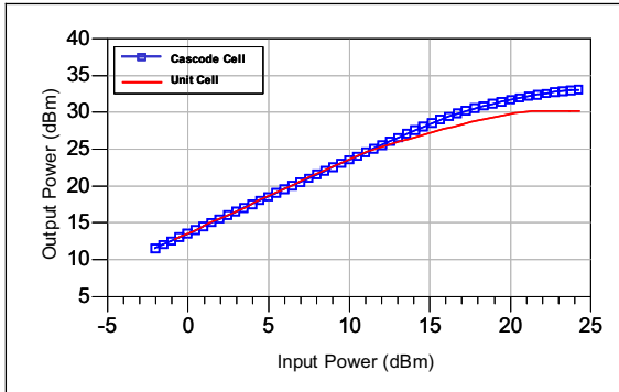
Fig. 7 Comparison of the output power versus input power for the cascode cell and a single transistor with input (Cag // Rag) cell.
