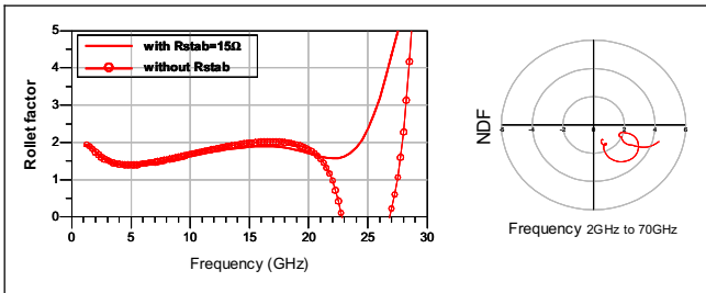
Fig. 2 (a) Influence of Rstab on Rollet factor (b) NDF of the cascode cell.
