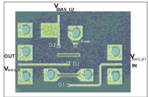
Fig. 4 Photograph of the AlN die designed to flip-chip the GaN cascode. (Input and output lines, DC bias paths, Electrical bumps, Via-Holes)
