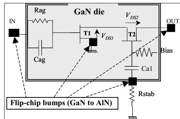
Fig. 1 Schematic of the power cascode cell (GaN die flip-chipped onto AlN)
