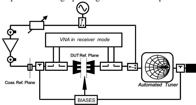
Fig. 10 On-wafer Pulsed Load-Pull Measurement Setup
