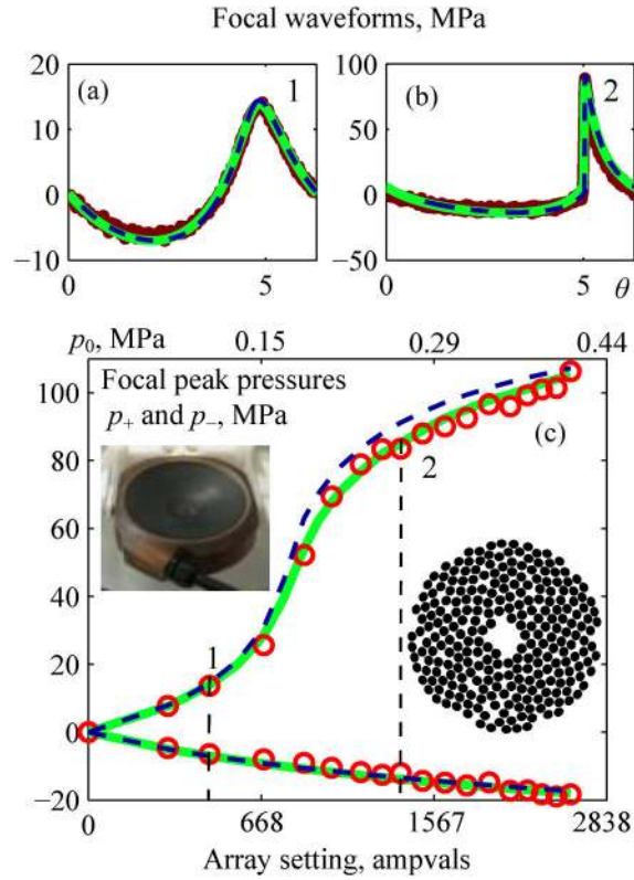
Fig. 15. Comparison of results for the nonlinear pressure field at the focus of a 1.2 MHz 256-element clinical array [27]. Measurement data (bold curves for the waveforms and circles for peak pressures) and results from KZK (dashed curves) and Westervelt (solid curves) models are shown for focal waveforms p_F(\theta) (a), (b) and for focal peak pressures as a function of the voltage V_0 applied to the transducer surface (c). Vertical dashed lines mark quasilinear (1) and developed shock (2) levels of distortion; corresponding waveforms (a) and (b) are shown above. Parameters of an equivalent single-element spherical source were determined as a = 6 cm, F = 11 cm, F_\# = 0.922 , ka = 301 .
