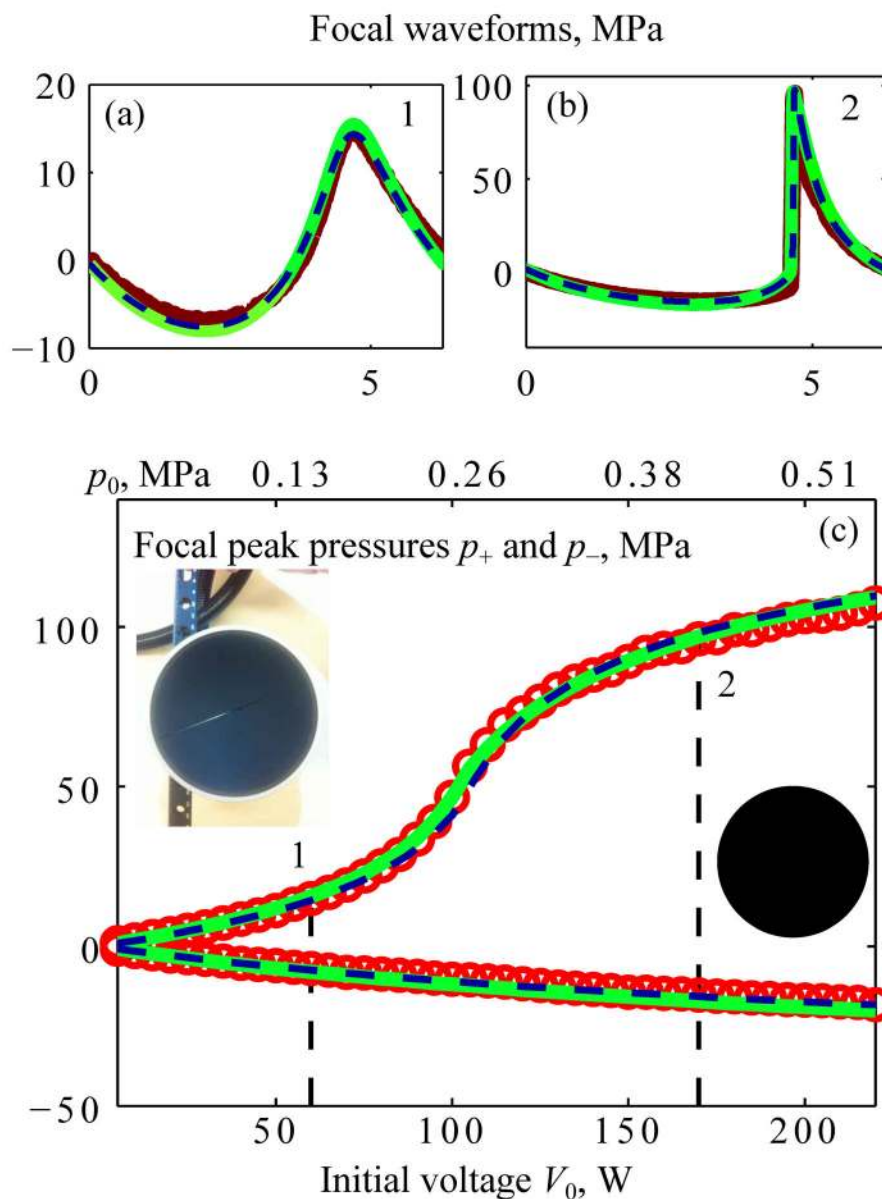
Fig. 13. Comparison of results for the nonlinear pressure field at the focus of a single-element spherical transducer of 1 MHz frequency, a = 5 cm radius; F = 9 cm focal length ( F\# = 0.9 , ka = 209 ) [25]. Measurement data (bold curves for the waveforms and circles for peak pressures) and results from KZK (dashed curves) and Westervelt (solid curves) models are shown for focal waveforms p_F(\theta) (a), (b) and for focal peak pressures as a function of the voltage V_0 applied to the transducer surface (c). Vertical dashed lines mark quasilinear (1) and developed shock (2) levels of distortion; corresponding waveforms, (a) and (b), are shown above. A photo and front view sketch of the transducer are also included in the figure.
