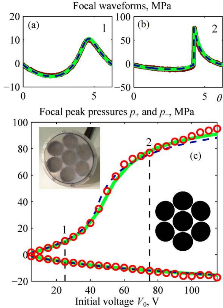
Fig. 14. Comparison of results for the nonlinear pressure field at the focus of a 1 MHz 7-element array [26]. Measurement data (bold curves for the waveforms and circles for peak pressures) and results from KZK (dashed curves) and Westervelt (solid curves) models are shown for focal waveforms p_F(\theta) (a), (b) and for focal peak pressures as a function of the voltage V_0 applied to the transducer surface (c). Vertical dashed lines mark quasilinear (1) and developed shock (2) levels of distortion; corresponding waveforms (a) and (b) are shown above. Parameters of an equivalent single-element spherical source were determined as a = 6.4 cm, F = 13.2 cm, F_{\#} = 1.03 , ka = 269 .
