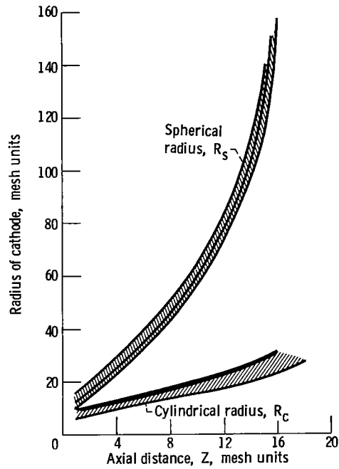
Figure 7. - Spherical radius of curvature computed from curve-fitted scalar magnetic potentials of ring pole piece.
