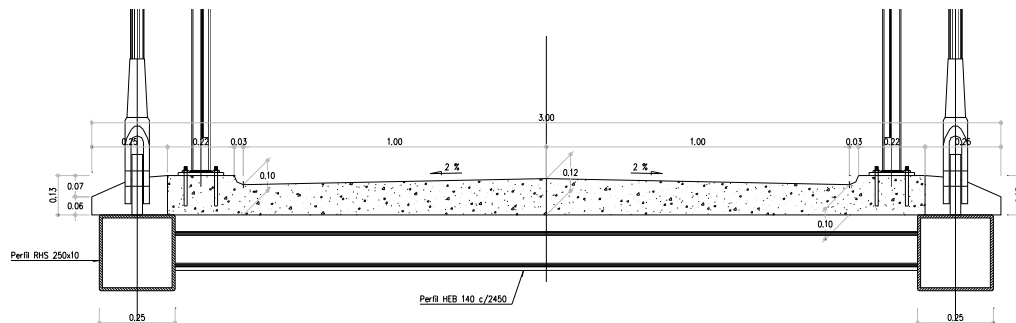
Figure 7-5: Cross section of Guarda Footbridge
