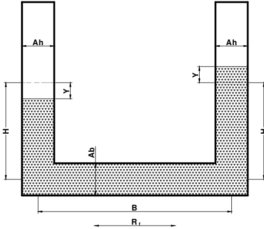
Figure 6-6: TLCD scheme
