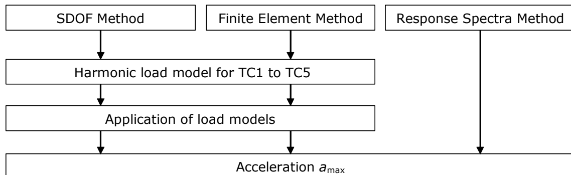
Figure 4-4: Methods for calculating the maximum acceleration
