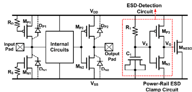
Fig. 1. Typical on-chip ESD protection scheme.
