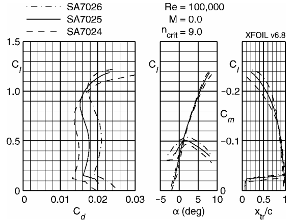
Fig. 9 XFOIL predictions for the SA702x airfoil series at Re of 100,000.
