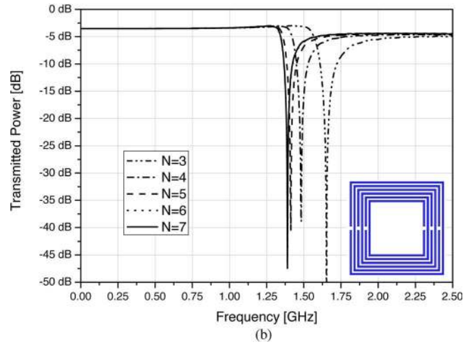
Fig. 9. Reflected and transmitted power from and through the absorber depicted in Fig. 8 for different values of the number of the rings N . The geometrical dimensions of the absorber are: l = 5 mm, w = 0.1 mm, s = 0.1 mm, g = 0.1 mm, p_h = 2 mm, p_v = 0.5 mm, d_f = 0.5 mm, and d_s = 0.5 mm. The total resistance of the resistive sheet is 377 \Omega .
