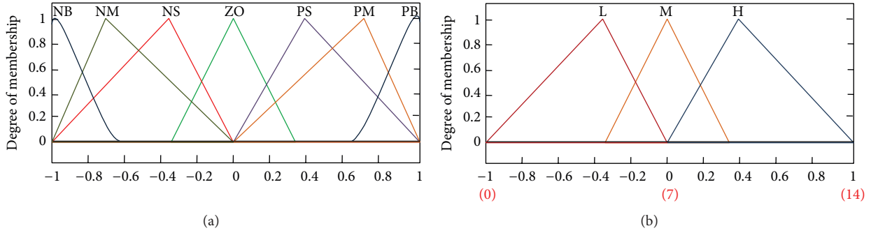
FIGURE 7: Membership functions for (a) e , de , K_p , K_I , and K_D ; (b) AV with normalised discourse.
