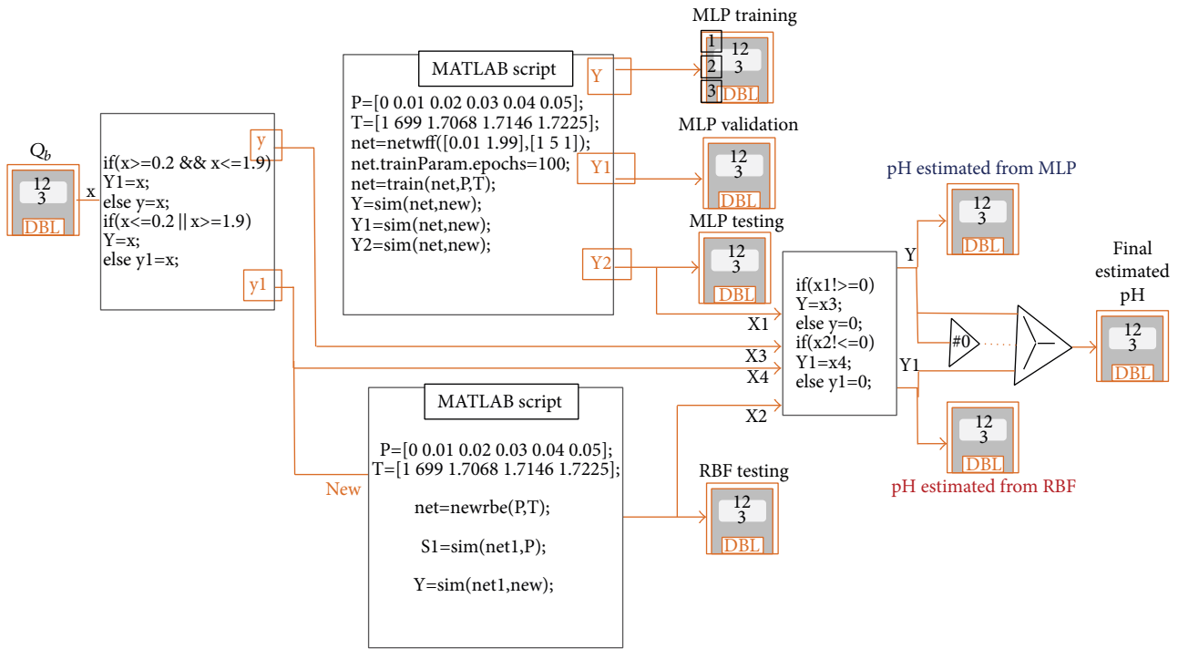
FIGURE 10: The MatLab script files of HNN in LabView.
