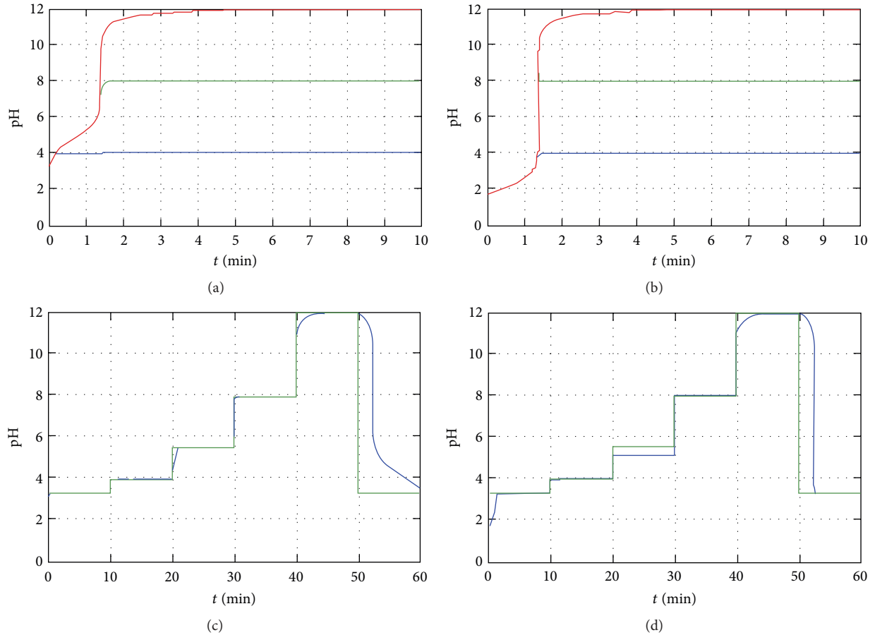
FIGURE 14: Performance of multiregional fuzzy PID controller in the three regions of titration curve for weak acid (a, c) and also for strong acid (b, d).
