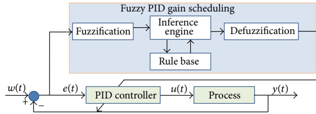
FIGURE 1: Structure of supervisory fuzzy PID.
