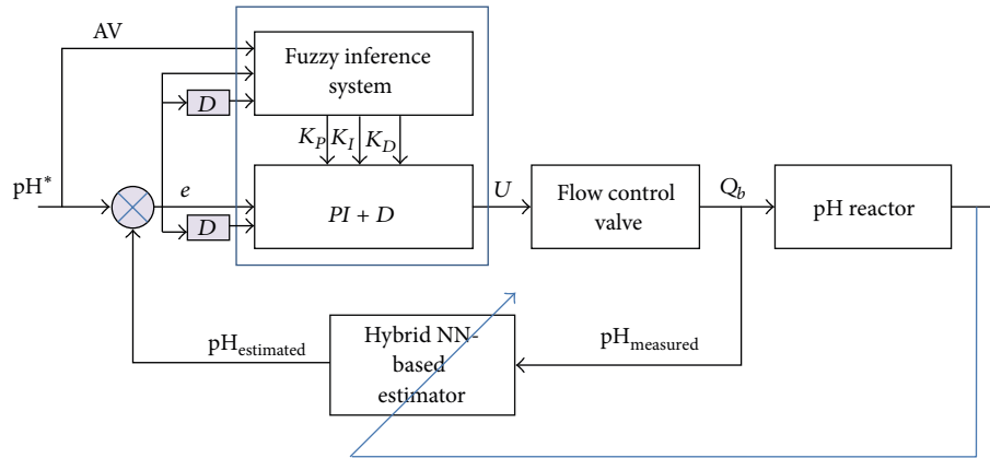
FIGURE 5: Supervisory fuzzy PID-based control over pH reactor.
