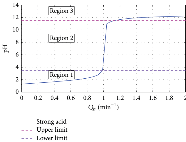
FIGURE 6: The titration curve subdivided into three regions.
