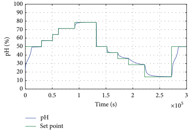
FIGURE 12: PID-controlled response.
