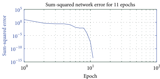
FIGURE 9: The SSE plot for the performance of the hybrid NN-based estimator.
