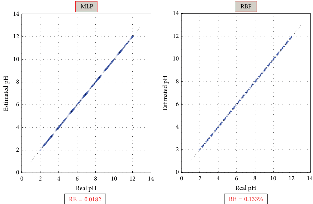
FIGURE 8: The computed relative error (RE) for both RBFNN and MLPNN.
