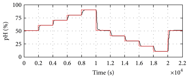
FIGURE 13: Supervisory fuzzy PID response process.
