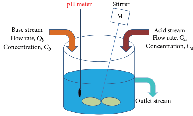
FIGURE 4: pH reactor.
