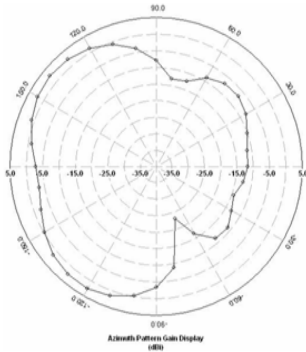
Fig. 12 Radiation Pattern at 3.54 GHz
