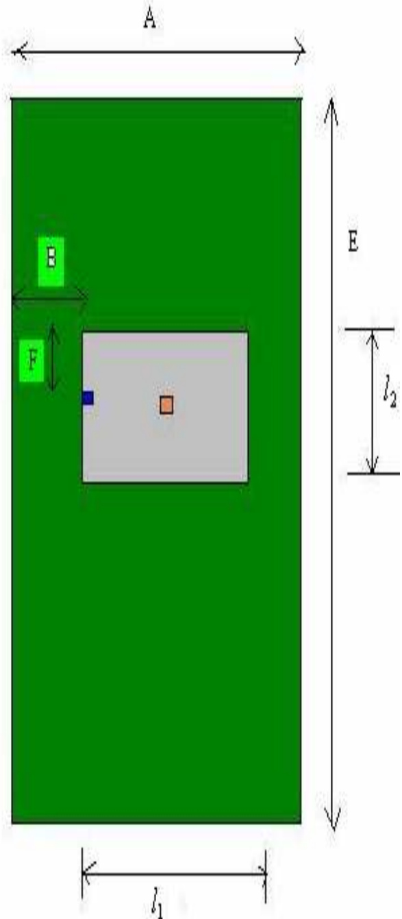
Fig.5 Proposed PIFA Antenna Structure
