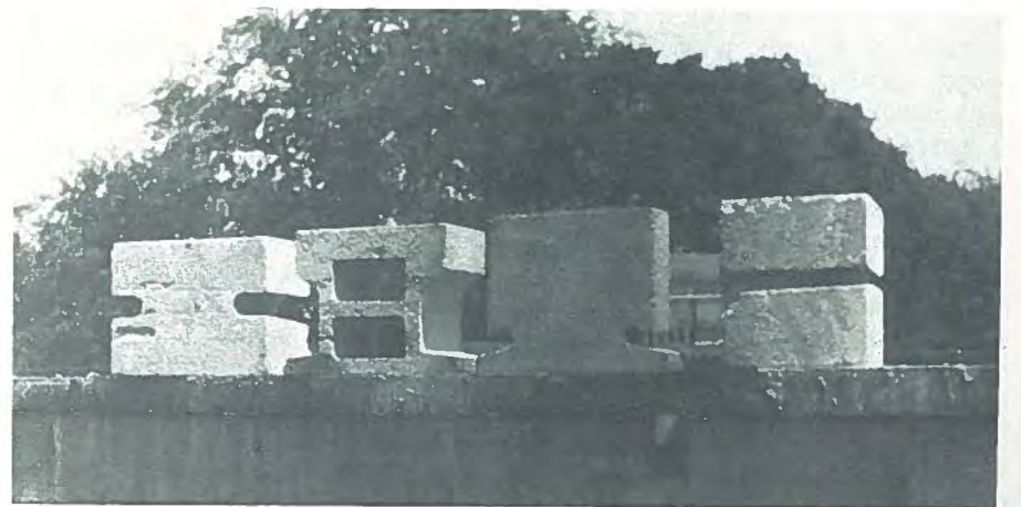
Fig. 5. Redesigned bridge beam units.
