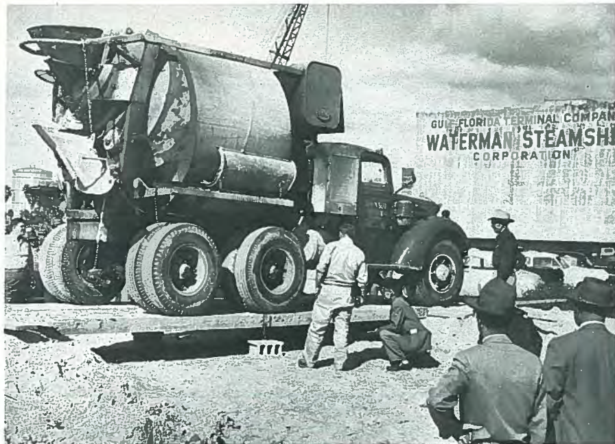
Fig. 24. Demonstration test by Cone Brothers Construction Co. in Tampa, Florida (1954) of 2-in. (51 mm) thick prestressed slab with 4-in. (102 mm) composite topping. The span was 30 ft (9.2 m) long.
