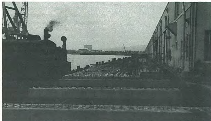
Fig. 55. All prestressed marginal wharf for railroad loading: prestensioned concrete piles, precast pretensioned cap girder, and precast pretensioned deck slabs to be part of lower portion of deck make up the structure. Cast-in-place concrete in upper part of deck ties together all the components of the wharf.
