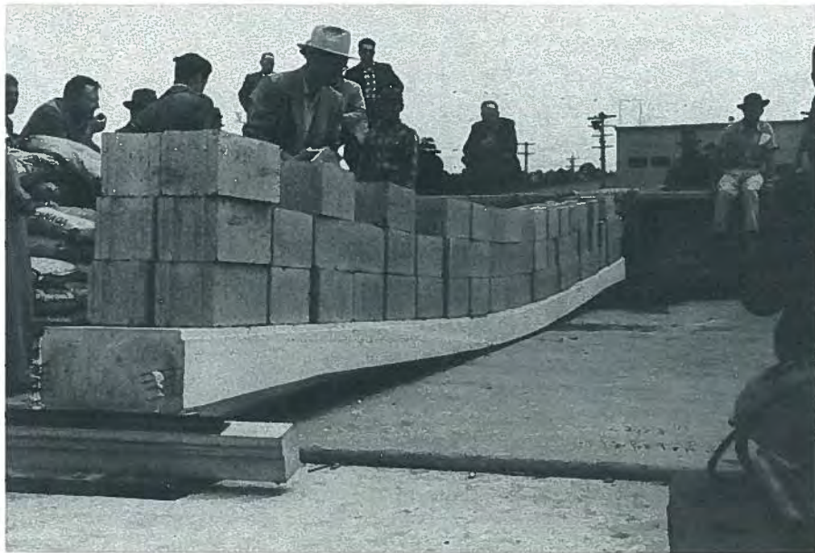
Fig. 6. Load test of prestressed concrete slab.
