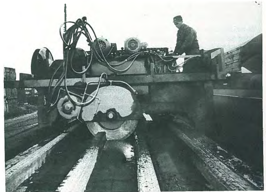
Fig. 26. After the concrete set, the Quadeck was cut to size by a saw attached to the machine.
