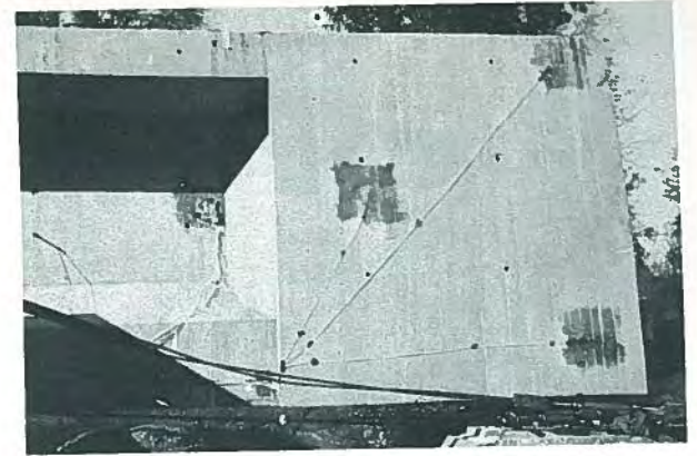
Fig. 9. East end of Walnut Lane test girder, looking north, showing strain gage installation on concrete.
