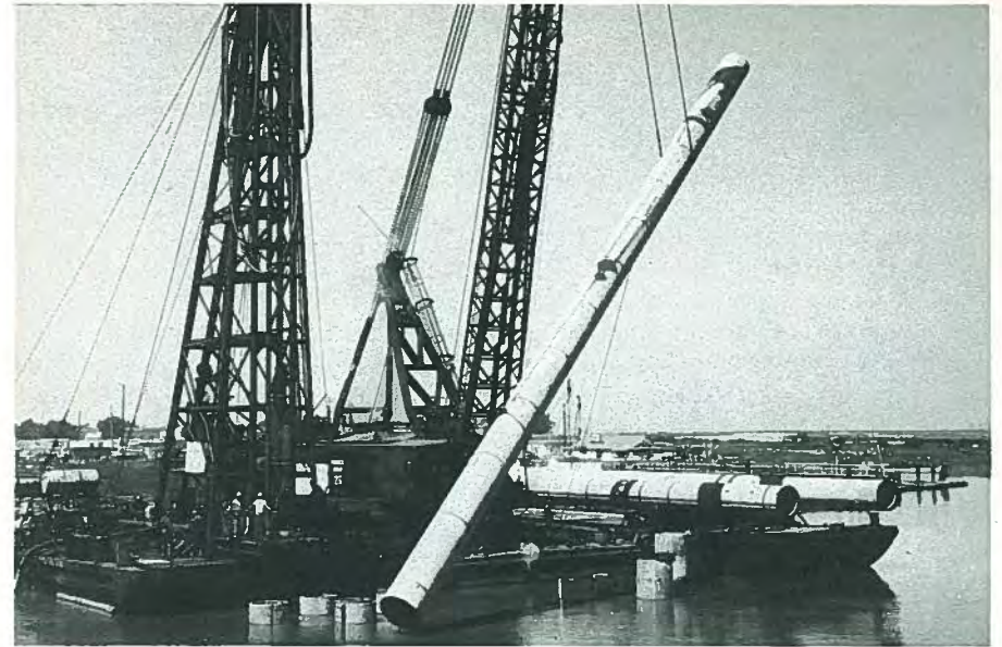
Fig. 52. Napa River Bridge, California: pretensioned monolithic cylindrical pile, 54 in. diameter, 120 ft long. It is believed to be the first such pile used worldwide.
