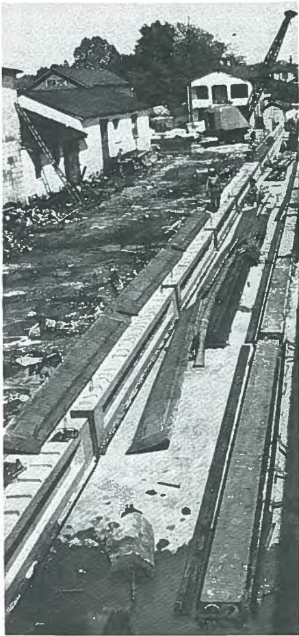
Fig. 12. Prestensioned bonded "I" section girders at casting plant in New Orleans for the production of girders for Loyola University's stadium about 1953.
