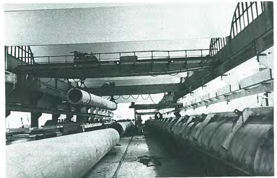
Fig. 84. Freshly cast prestressed hollow cylinder piles.
