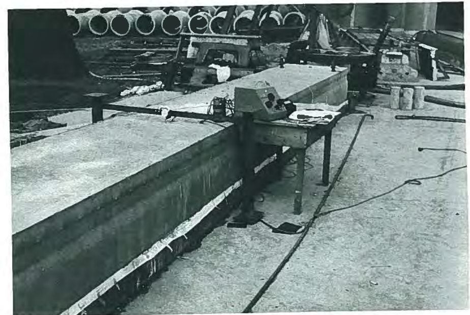
Fig. 21. Strainmeter setup for measuring strains during prestressing operation.
