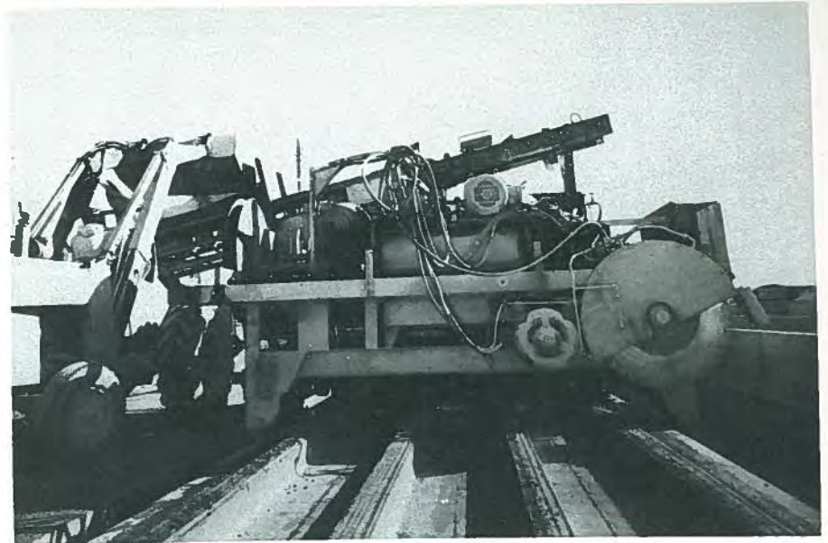
Fig. 25. In 1961 Jack Perlmutter developed a hydraulically-operated horizontal slip form machine to cast a Quadeck, an inverted tee slab with four stems. A front end loader charged the hopper on the Quadeck slip form.
