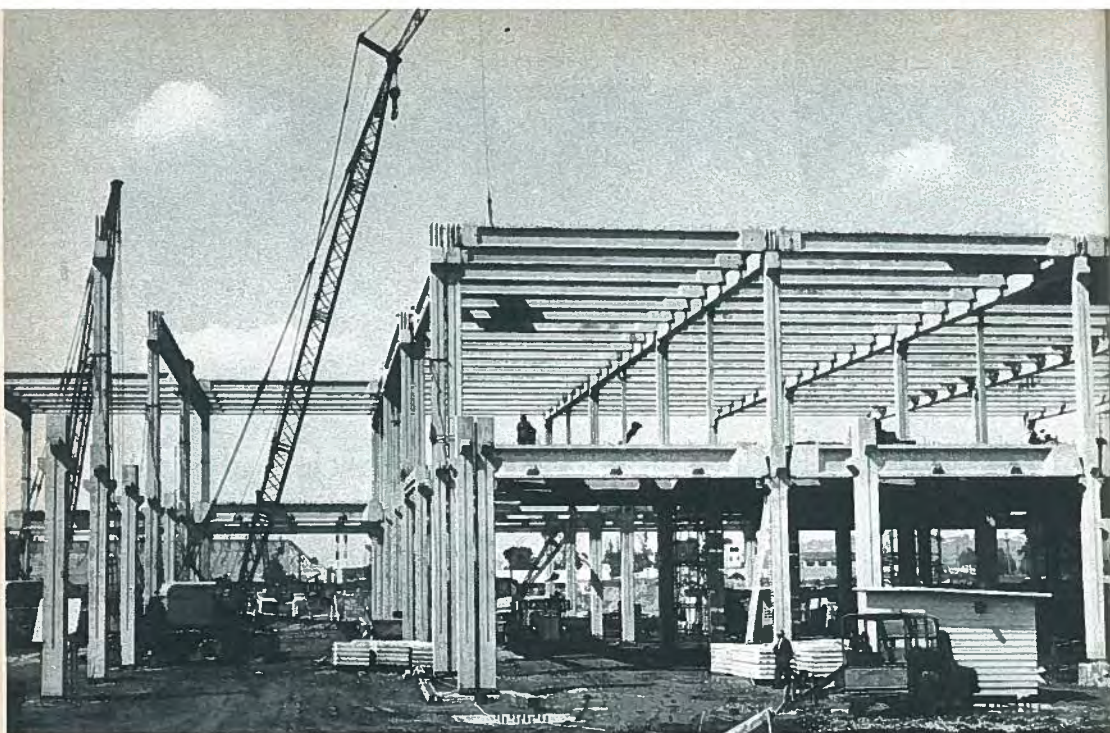
Fig. 42. Erection of giant Boeing Company development center in Seattle, Washington, 1956. The two-story 400 x 600 ft (122 x 183 m) precast prestressed structure with 40 x 60 ft (12.2 x 18.3 m) bays was completed in 7 months and at the time was the largest industrial-type prestressed building in the world.
