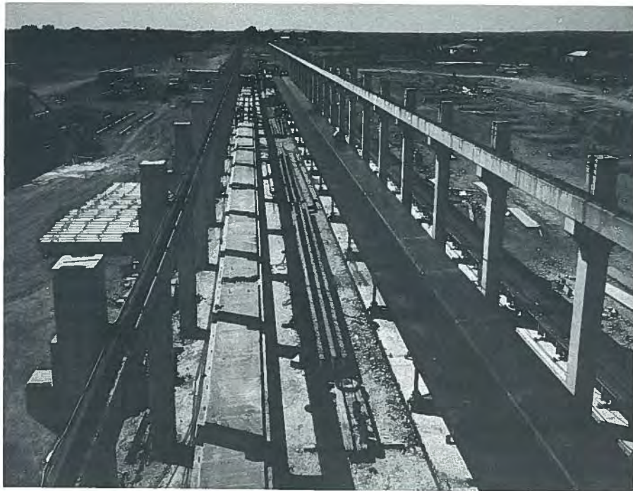
Fig. 11. The modern plant of Wilson Concrete Products under construction (1956).
