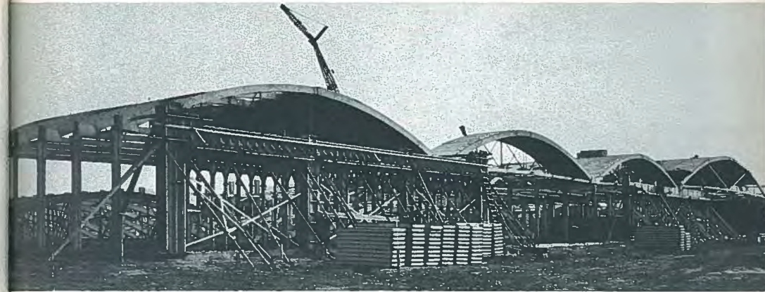
Fig. 13. Segmented prestressed bow-string trusses for the Birchmount garage of the Toronto Transportation Commission.
