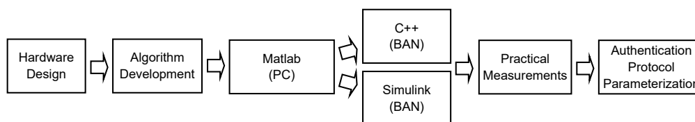
Figure 3. Development flow.
