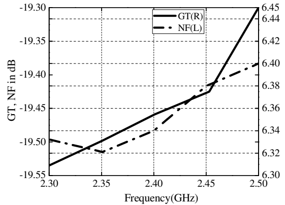
Fig.8. NF & GT of Sequential Fed Balanced Amplifying CP Antenna
