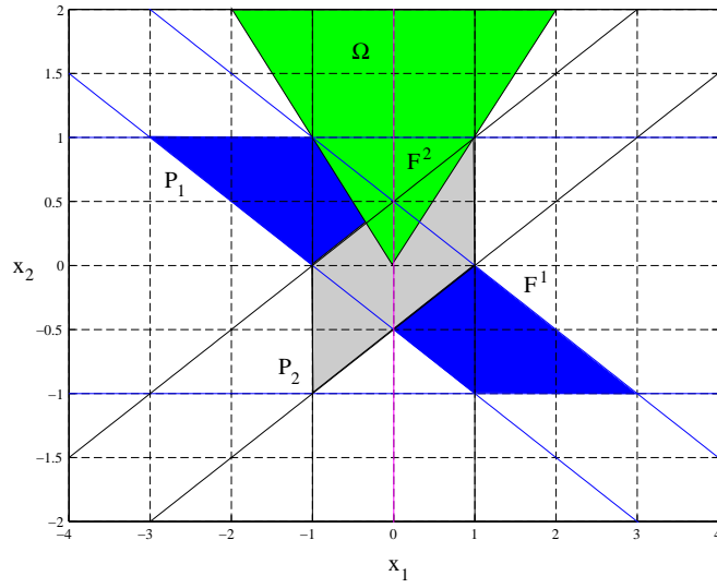
Figure 4: The region \Omega .
