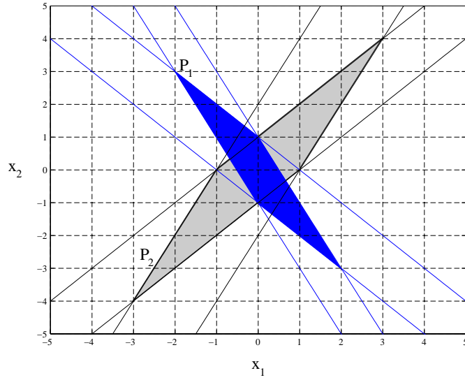
Figure 8: Positively invariant polyhedral sets.
