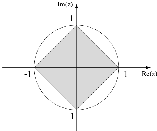
Figure 2: Eigenvalue locations in the complex plane.
