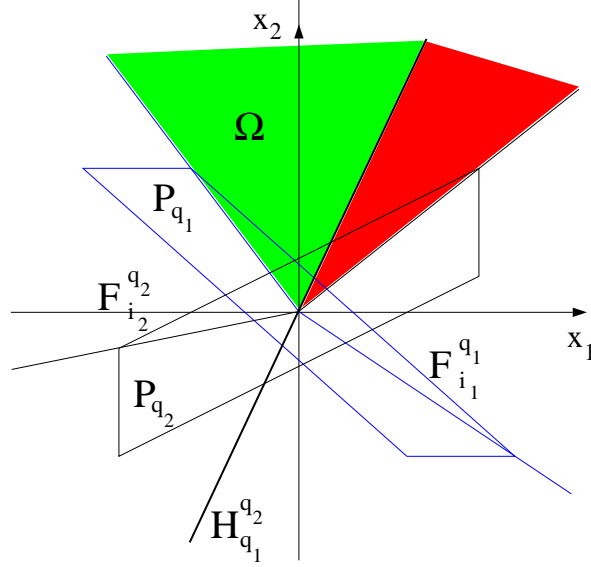
Figure 3: The conic partition of the state space.
