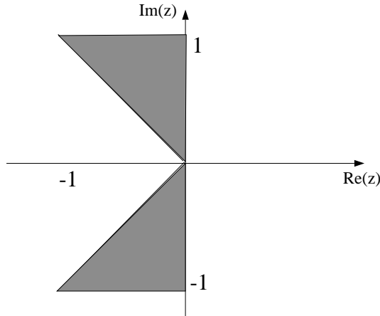
Figure 7: Eigenvalue locations in the complex plane.
