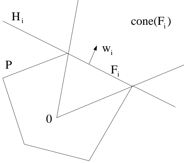
Figure 1: A polytope P , a face F_i and its corresponding hyperplane H_i .
