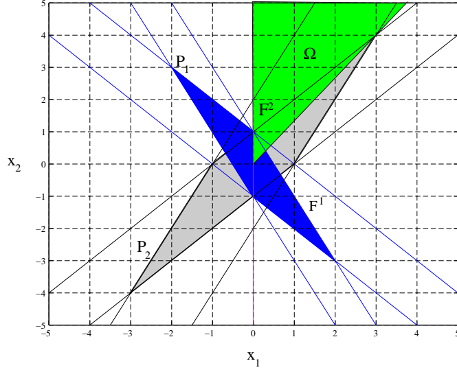
Figure 9: The region \Omega .
