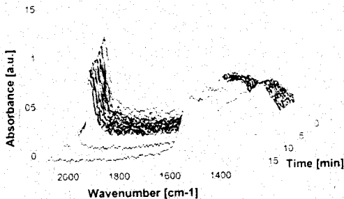
Figure 3 Time resolved IR spectra during CO 2 adsorption on Pt/ZrO 2 . T=775K, pCO 2 =0.25, total flow 30ml/min -1
