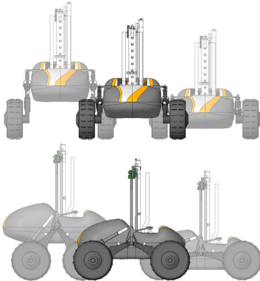
Figure 5: High, nominal and low ride heights
