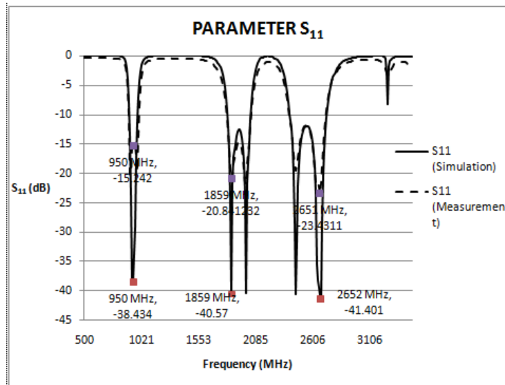
Figure 6 S_{11} results of the fabricated BPF using cascade TSSIR.
