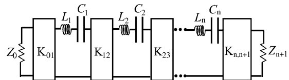
Fig. 2. Generalized bandpass filter network with impedance inverters and series LC resonators.
