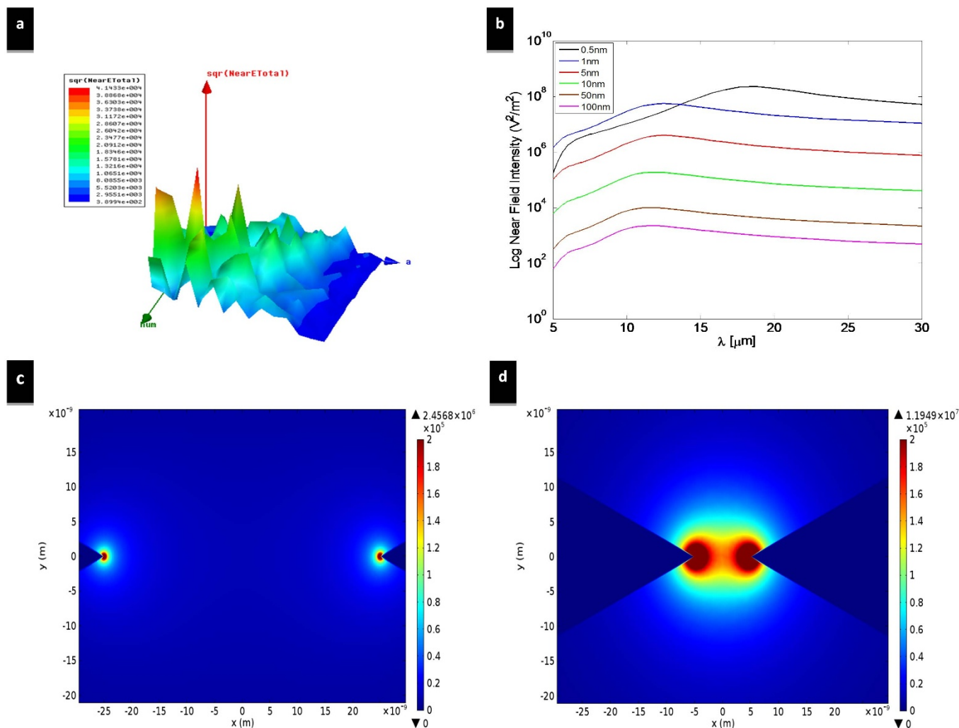
Figure 3 | Nano antenna optimization and near-field intensity variation with gap size. (a) The near field intensity enhancement for several bowtie antennas with a gap of 50 nm is plotted against antenna length (green axis) and half bow angle (blue axis). For a gap of 50 nm, an enhancement factor of 4 \times 10^4 was achieved for 2.7 \mu\text{m} length and 50^\circ bow angle. (b) Numerical simulation of the optimized bowtie dipole versus different gap sizes. The plotted relative intensity enhancement is defined as the ratio between the electric field intensity at the middle of the gap to the electric field intensity of the incident plane wave. (c) Simulated relative near field intensity enhancement for the optimized bowtie of a 50 nm gap. (d) Simulated relative near field intensity enhancement for the optimized bowtie of a 10 nm gap.
