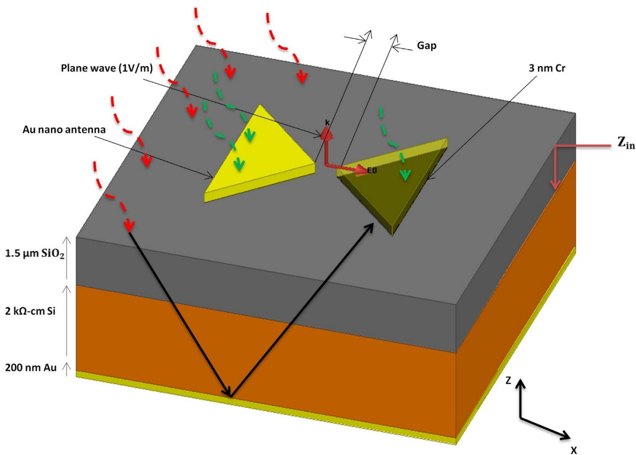
Figure 1 | Device structure. Gold nano antenna of 100 nm in thickness is mounted on 3 nm of chromium adhesion layer. The gap size ranges from 100 nm to 0.5 nm. The substrate is made of 1.5 \mu\text{m} of silicon dioxide that acts as a matching section, 375 \mu\text{m} high resistivity silicon, and finally 200 nm of gold to function as a back reflector. Excitation is through an incident plane wave with electric field intensity of 1 V/m. Z_{in} is the input impedance to the waves impinging on the silicon dioxide matching section (red arrows). The black arrow represents substrate coupling by the reflected waves. The green arrow represents the waves coupled to the antenna.
