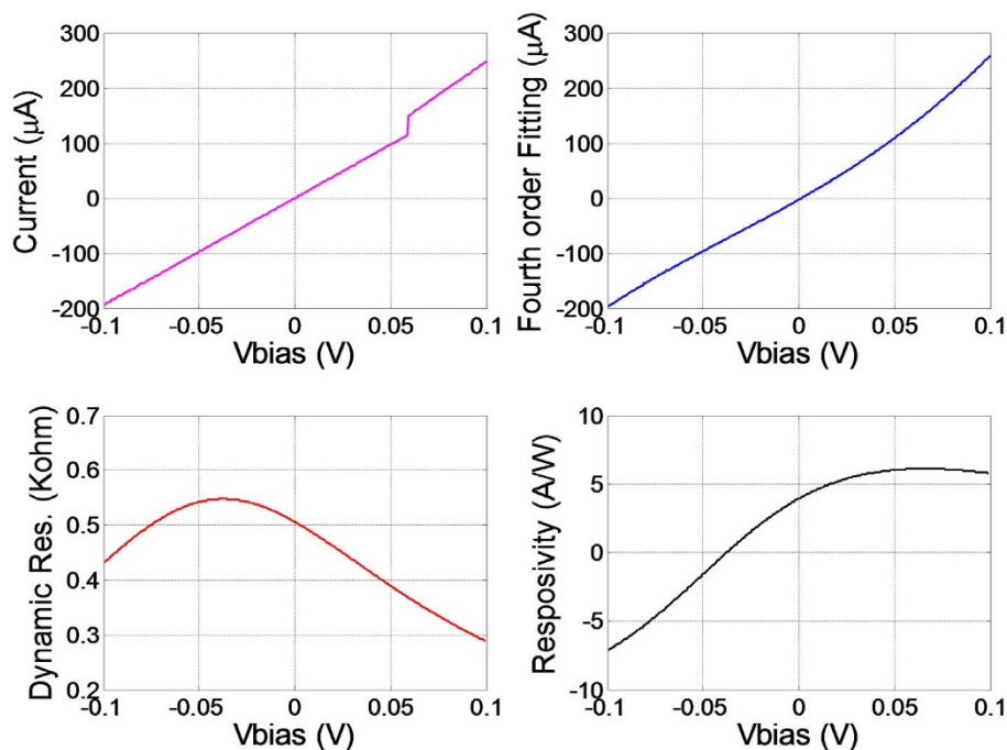
Figure 5 | Rectenna device performance. (a) The I - V characteristics of the MIM diode. (b) Fourth-order fitting of the I - V curve. (c) The diode's dynamic resistance with a value of 500 \Omega at zero bias. (d) Responsivity with a value of 4 \text{ A/W} at zero bias and maximum value of 6 \text{ A/W} at 0.1 \text{ V} .
