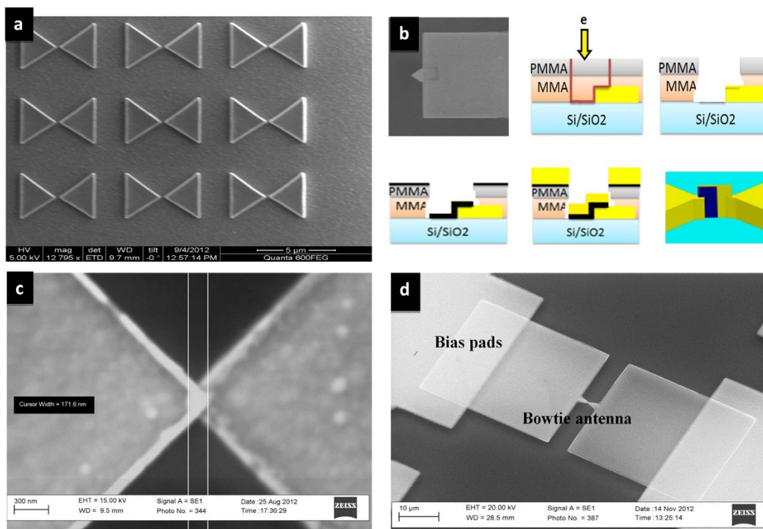
Figure 4 | Fabrication of nano antennas and the rectenna device. (a) SEM image of the nano antenna array fabricated using EBL. (b) Overlap fabrication process: (i) First antenna arm, (ii) Second arm exposure using EBL, (iii) Removing the exposed resist using a mixture of MIBK and IPA developer with ratio of 1:3, (iv) Deposition of 0.7 nm of oxide using atomic layer deposition (ALD), (v) Second arm sputtering, (vi) Complete device after the liftoff process using acetone. (c) SEM image of the fabricated overlap. (d) SEM image of the antenna-integrated diode. The lower arm is made of 95 nm of gold over a 5 nm chromium layer, while the upper arm is made of 100 nm of copper. The tips of both arms sandwich 0.7 nm of copper oxide. Bias pads ( 20 \mu\text{m} \times 32 \mu\text{m} ) are connected to the antenna for diode bias and signal readout purposes.
