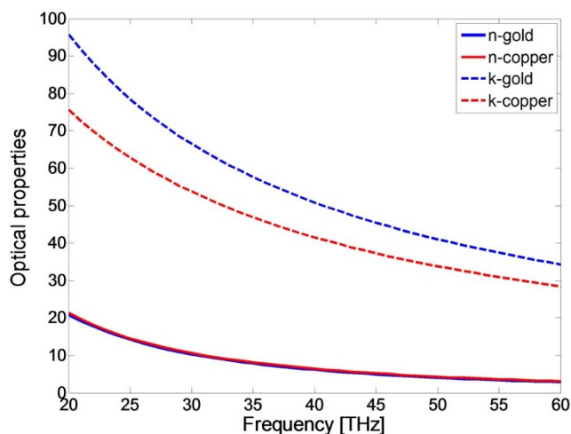
Figure 2 | Frequency dependent optical properties of thin film gold and copper. Experimentally measured complex refractive index for thin film (75 nm), gold (blue line), and copper (red line). Gold and copper have the same frequency dependent refractive index, but the higher value of gold's extinction coefficient indicates higher absorption in THz frequencies.
