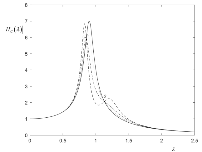
FIG. 6. Frequency response curves |H_C(\lambda)| using the proposed damping absorber (model C) with \mu = 0.15 , M = 100 kg, and \omega_n = 10 Hz. \gamma = 1 at \lambda = 1 with k = 0 (—); k = 0.2vG_{s-\omega_n} (···); k = 0.4vG_{s-\omega_n} (---), and k = 0.6vG_{s-\omega_n} (- · -). Pseudo fixed points P and Q are marked with •. The viscoelastic damper material used in model C has stiffness and loss factor as shown in Fig. 5.
