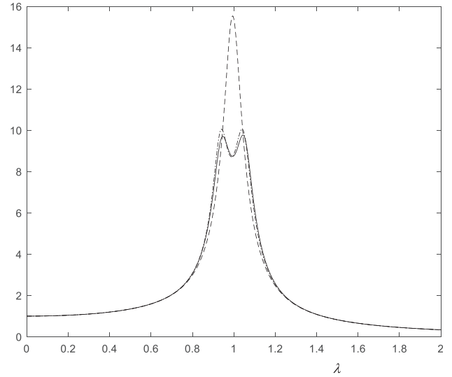
FIG. 10. Frequency response curves of the primary mass M with the optimized traditional DVA, |H_A(\lambda)| (model A, - - -), and the optimized model B, |H_B(\lambda)| (model B, - · -), and the proposed optimized VDVA, |H_C(\lambda)| (model C, —). \mu = 0.02 , M = 100 kg, and \omega_n = 10 Hz. The viscoelastic damper material used in model B and model C has modulus and loss factor as shown in Fig. 9.
