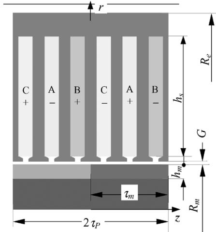
Fig. 8. Finite-element model.
