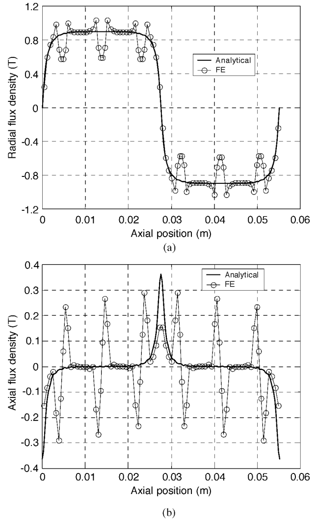
Fig. 9. Comparison of flux density in air gap as a function of z at r = 0.0473 , for z_d = 0 . (a) Radial component. (b) Axial component.
