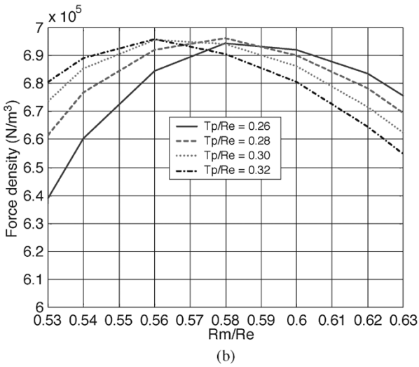
Fig. 15. Variation of force density with R_m/R_e and \tau_p/R_e . (a) 3-D view. (b) 2-D view.
