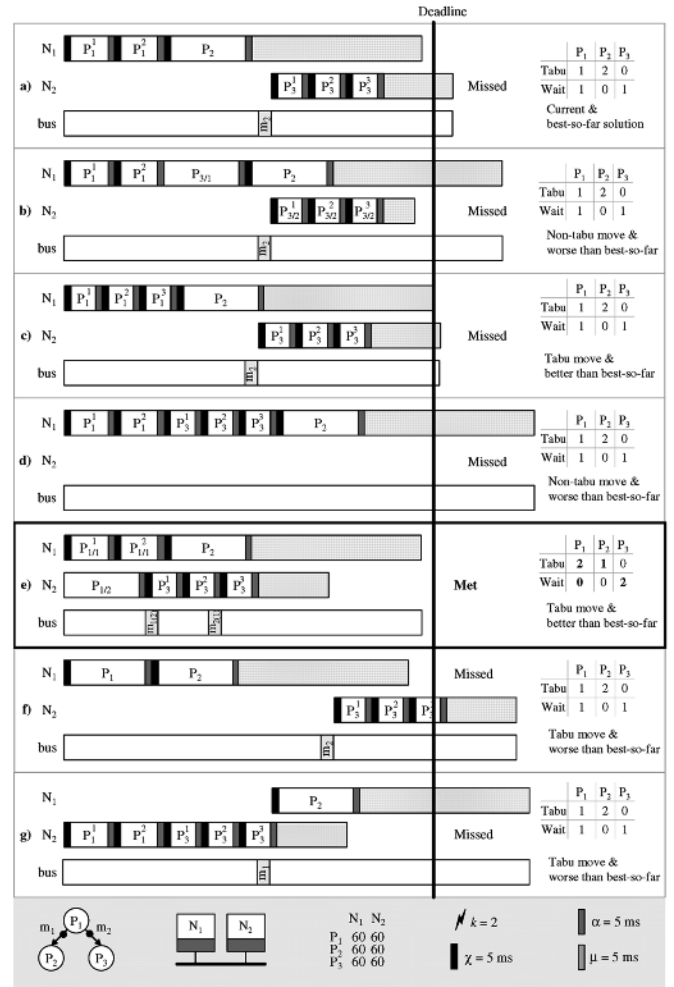
Fig. 10. Moves and Tabu History. Considering (a) as the current solution, the neighborhood is formed by (b)–(g).
