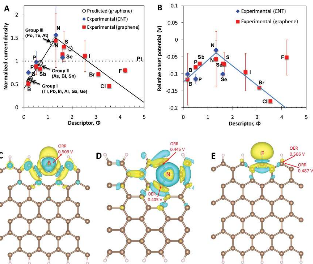
Figure 3. A) Measured limiting current density from the LSV curves, normalized by Pt/C electrode current density at 0.5 V (SCE, saturated calomel electrode) under the same conditions in the same experiment, and the predictions, and B) measured relative onset potential (difference between the doped carbon nanomaterials and the Pt/C electrode), as a function of descriptor, \Phi for p-element-doped carbon nanomaterials. The average current density is cited for graphene doped with B, [4,8] P, [10,35] N, [6,12,15] S, [13] F, [14,15,36] Cl, [17] Br, [17] I, [17,19] Se, [20] and Sb, [22] and for CNT doped with B, [9] P, [11,18] N, [16,18,21,30,37] and Se. [20] The predictions are based on the fitting lines of the experimental results. Differential charge density distributions (between doped and undoped graphene) of C) boron, D) nitrogen, and E) fluorine doped graphene sheets. The active sites with the minimum overpotential are marked with values. Yellow and blue colors indicate the positive and negative values of electron quantities, respectively. The isosurface value is set to 0.0015. Brown and white balls refer to carbon and hydrogen atoms, respectively.
