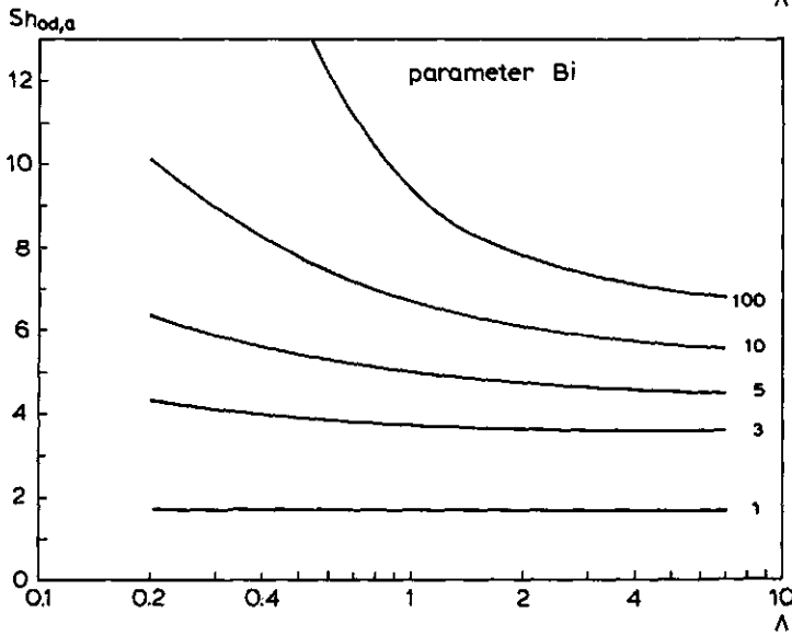
Fig. 24. Asymptotic Sh_d and Sh_{od} values for countercurrent extraction of spherical particles. Bi = mk_cR/D_d is the Biot number.
