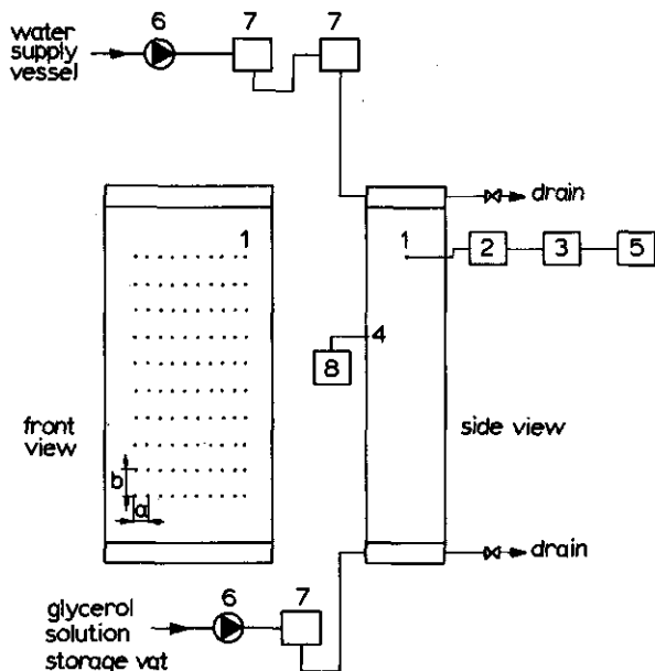
Fig. G1. Schematic picture of the experimental setup.
