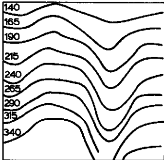
Fig. G3. Front positions under slightly unstable displacement conditions. M = 20 ; \langle v \rangle / v_c = 5 ; \langle v \rangle = 6.2 \times 10^{-8} m/s; Parameter time.
