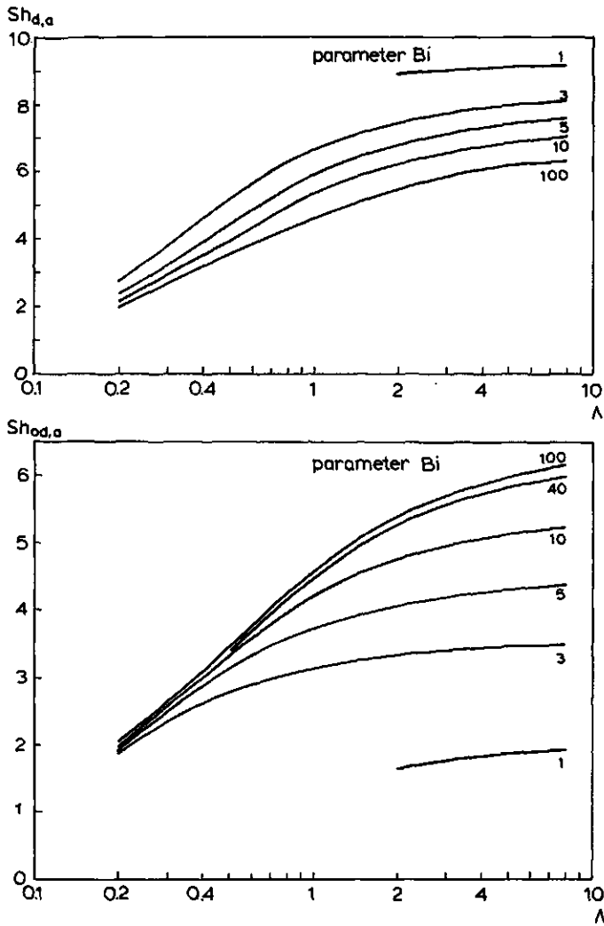
Fig. 27. Asymptotic Sh_d and Sh_{od} values for cocurrent extraction of spherical particles. Bi = mk_cR/ID_d is the Biot number.
