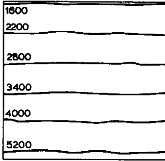
Fig. G2. Front positions under stable displacement conditions. M = 60 ; \langle v \rangle / v_c = 0.6 ; \langle v \rangle = 0.33 \times 10^{-4} m/s; Parameter time.
