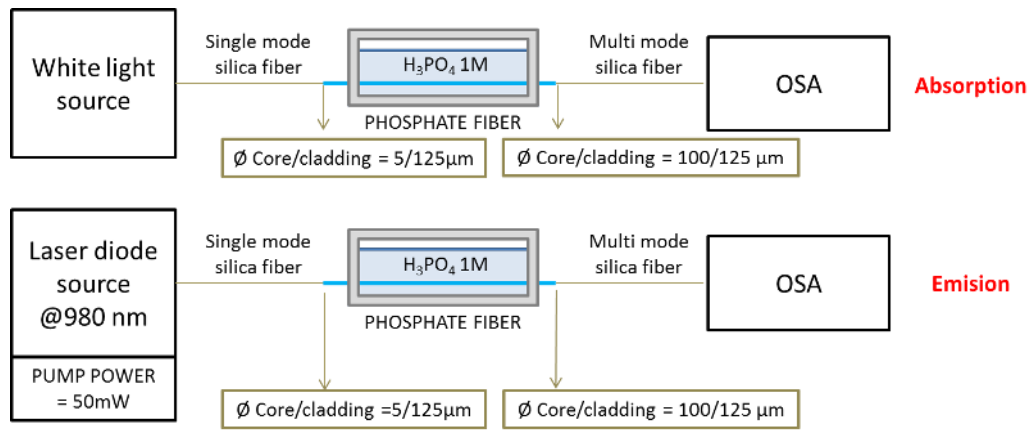
Figure 3.22 Schematic representation of the set-up used for the emission and absorption measurements of the fiber immersed in \text{H}_3\text{PO}_4 1M solution
