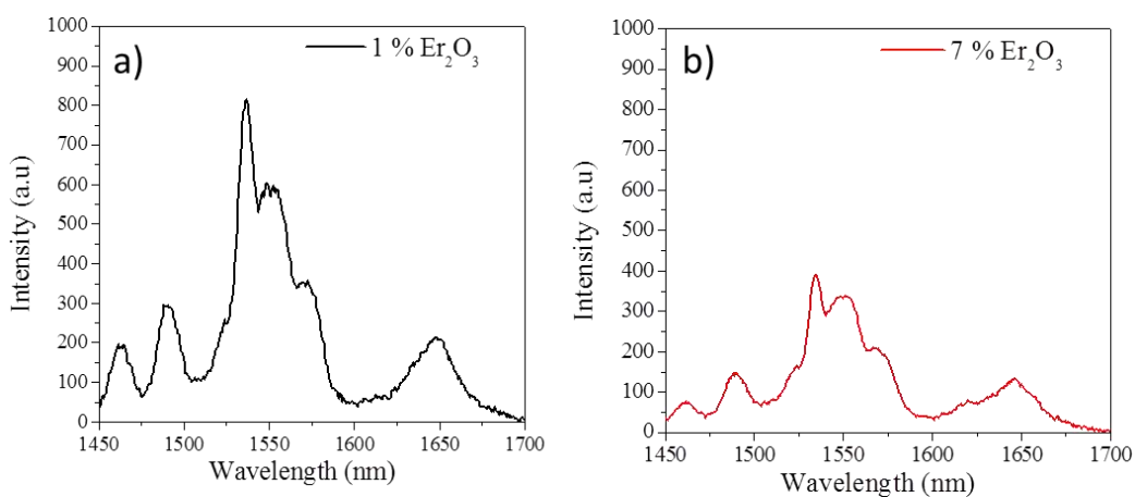
Figure 4.17 Emission spectra of (a) 1 and (b) 7 mol% \text{Er}^{3+} -doped \text{Al}_2\text{O}_3 particles calcined at 1300^\circ\text{C} for 5h.
