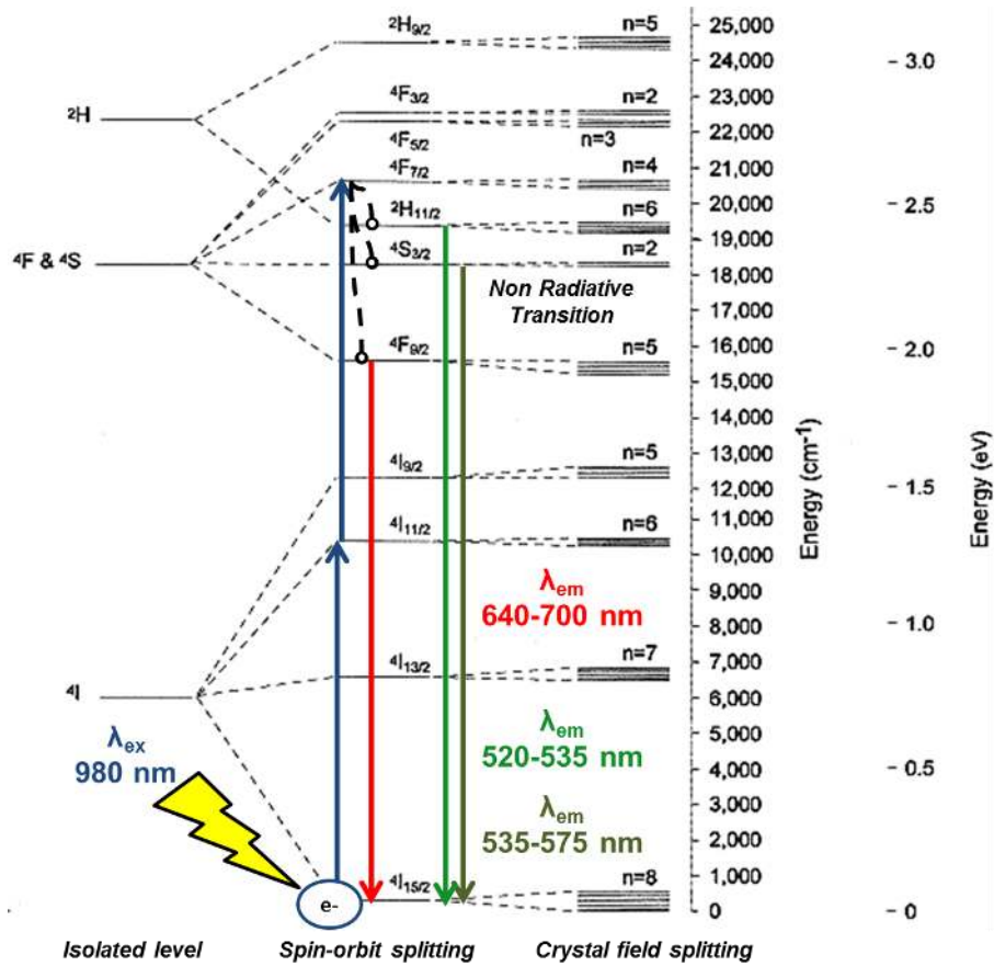
Figure 2.9 Up-conversion mechanisms in an Er 3+ -doped material. Figure modified from [118] and [103].
