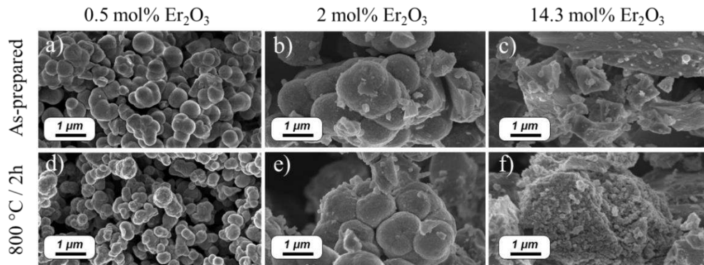
Figure 4.19 FE-SEM micrographs of 0.5, 2 and 14.3 mol% \text{Er}_2\text{O}_3 -doped \text{TiO}_2 particles as-prepared (a, b, c) and calcined at 800 °C for 2 h (d, e, f), respectively.
