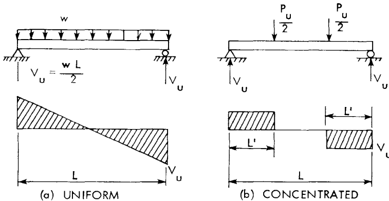
Fig. 7. Uniform and concentrated load application.
