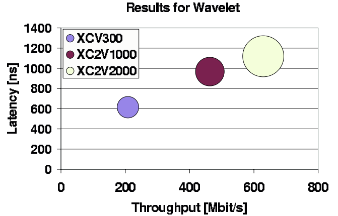
Figure 4: Results for the Wavelet design space exploration showing the best performers for each of the three FPGA sizes. The size of the circle indicates the area of the design.
