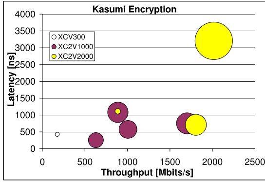
Figure 5: Kasumi design space exploration with ASC.
