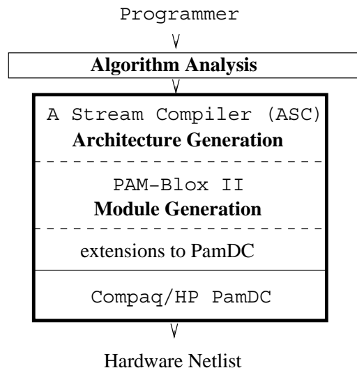
Figure 2: Levels of abstraction and structure of ASC. The bold box represents a single C++ program.
