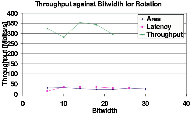
Figure 7: Bitwidth / Throughput tradeoff.
