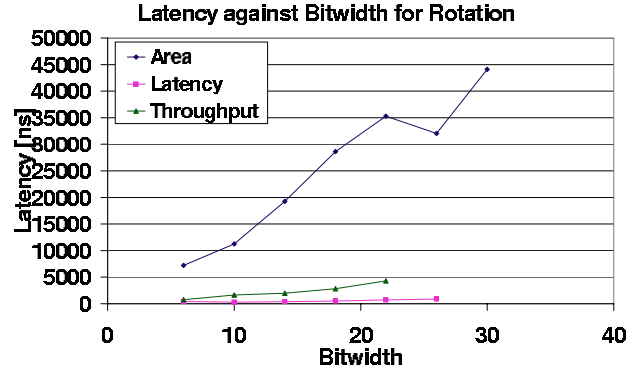
Figure 8: Bitwidth / Latency tradeoff.
