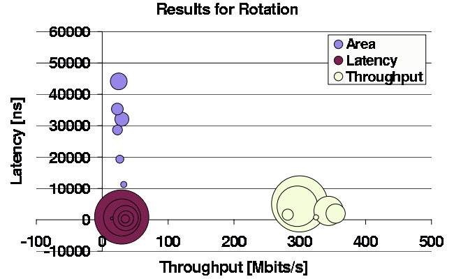
Figure 6: Rotation example, exploration of design space.
