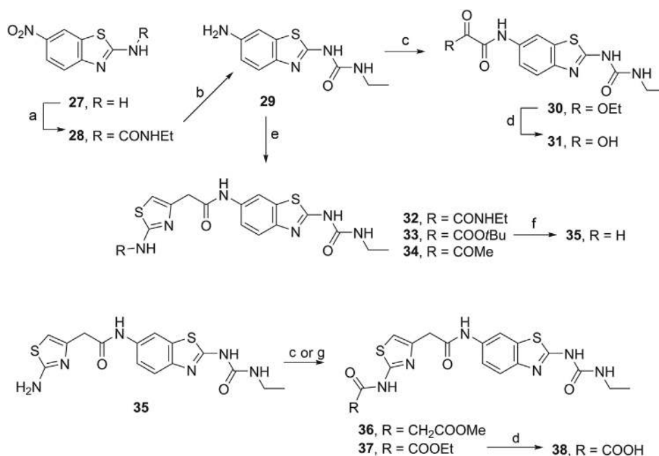
SCHEME 3 Synthesis of compounds 28–38. Reagents and conditions. a) Ethyl isocyanate, \text{Et}_3\text{N} , toluene, reflux, 24 h. b) \text{H}_2 , Pd/C, \text{EtOH}/\text{DMF} , r.t., 48 h. c) Ethyl oxalyl chloride, \text{Et}_3\text{N} , 1,4-dioxane, r.t., 18 h. d) 1 M NaOH, \text{MeOH}/\text{H}_2\text{O} , r.t., 18 h. e) Carboxylic acid, EDC, HOBT, NMM, DMF, r.t., 18 h. f) Acetyl chloride, \text{MeOH} , 0^\circ\text{C} , 1 h, then r.t., 18 h. g) Methyl malonyl chloride, \text{Et}_3\text{N} , 1,4-dioxane, r.t., 18 h
