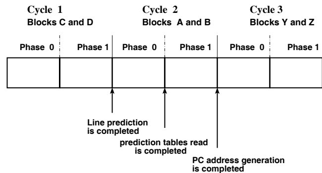
Figure 1. PC address generation pipeline
