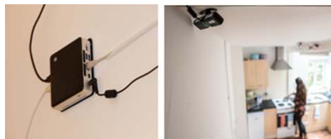
Figure 2. NUC and Asus Xtion sensor in SPHERE house.
