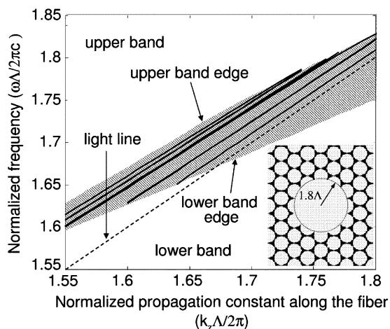
Fig. 3. Dispersion curves of the defect modes for a core radius R = 1.8\Lambda .
