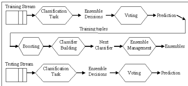
Figure 2: Generalized Boosting
