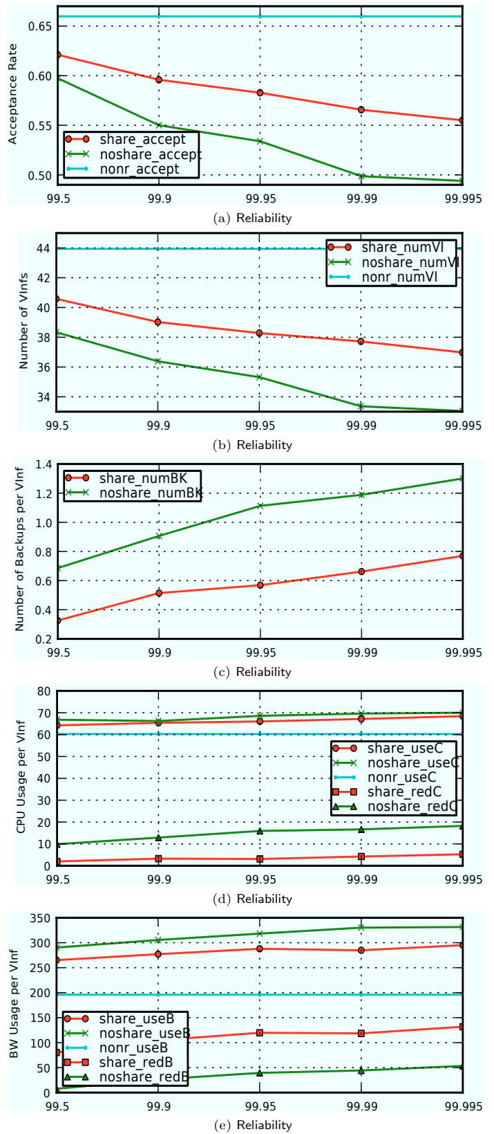
Figure 7: Figures above compare the performance of the system when backup nodes and links are shared against unshared. This is studied under varying reliability guarantees. nonr is the baseline case where VInfs are admitted without any redundancy.
