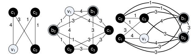
(a) VInf with three critical links for VInf with two backups. (b) Least number of critical links for VInf with two backups. (c) Addition of redundant (bold) links L to VInf for two backups.
