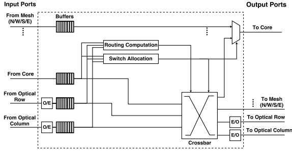
Figure 12: Router Architecture
