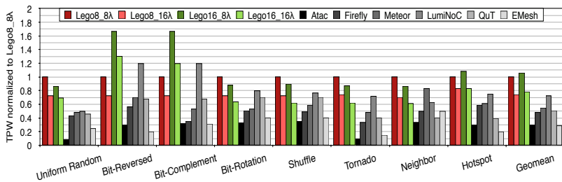
Figure 15: Normalized Throughput-per-Watt
