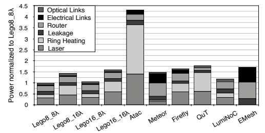
Figure 16: Power breakdown
